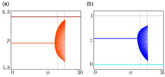
Figure 6. The asymptotic values of (a) p (orange and dark red) and (b) z (blue and cyan) versus \phi . The other parameters are a = 6 , b = 1 , \beta = 0.1 , \gamma = 0.289 , \delta = 0 , \rho = 0.3 , \eta = 0 .
